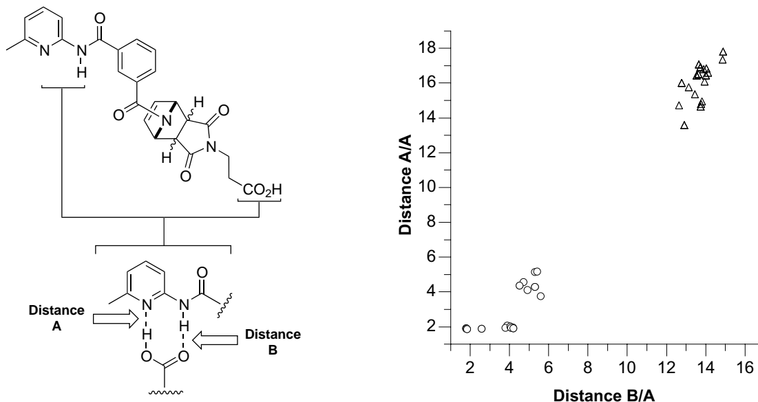
Figure 2. Structures of the 30 lowest energy conformations of exo -7 and endo -7 expressed as a function of key hydrogen bond distances. Open circles represent the location of conformations of exo -7 and open triangles represent the location of conformations of endo -7.
